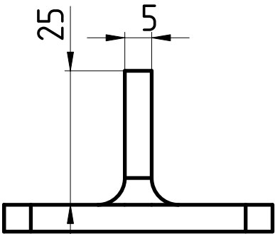
Left view
